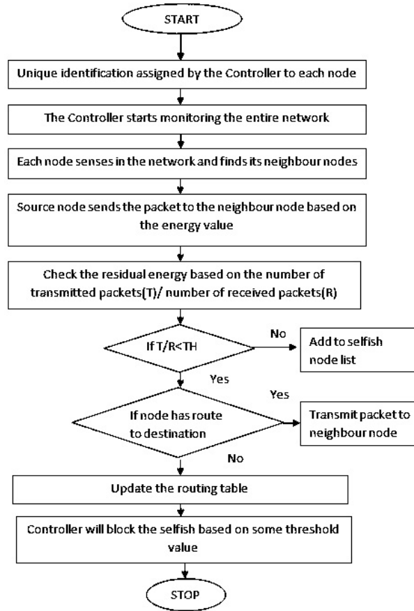
Fig. 3. Flowchart of the Overall Proposed System.
